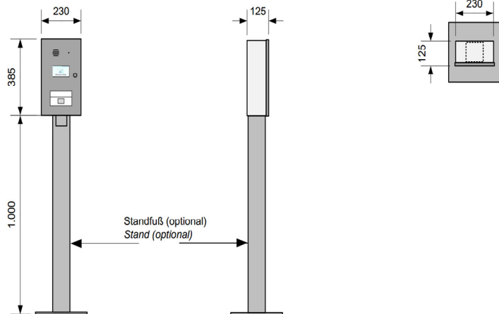
Vorderansicht be.Access Gate Front view be.Access Gate
